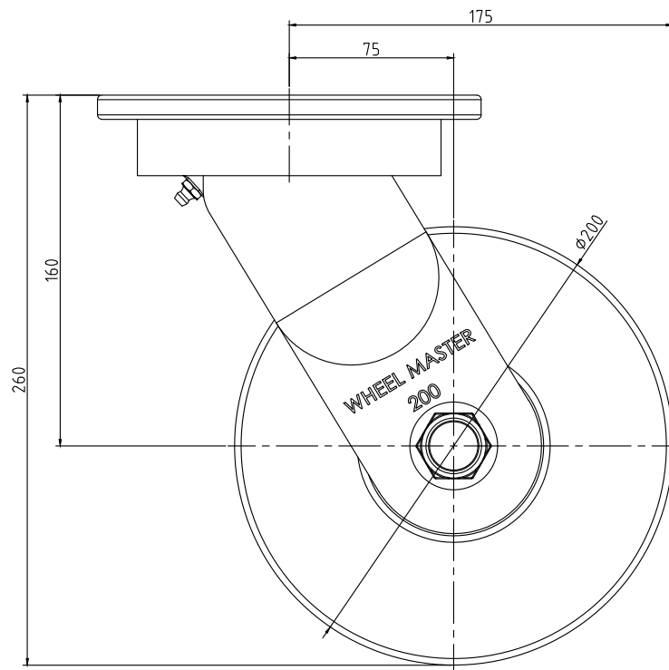
WXT-200SF
