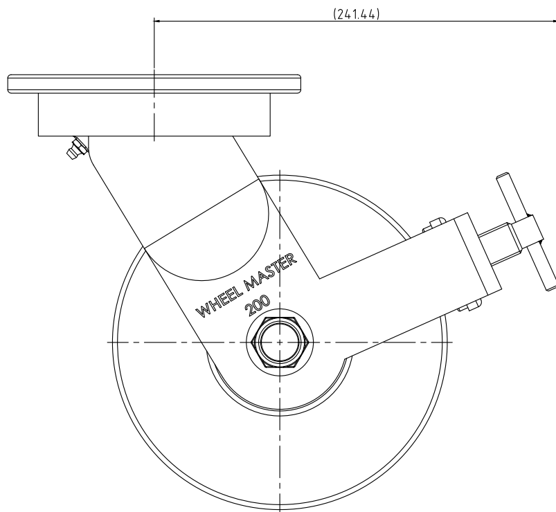
WXT-200SFBK-TYPE A
