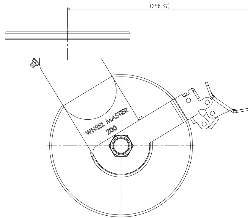
WXT-200SFBK-TYPE B
