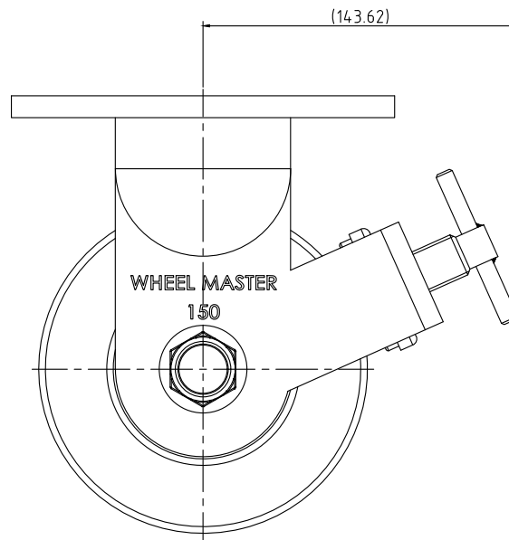
WXT-150RFBK-TYPE A
