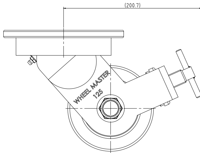
WXT-125SFBK-TYPE A
