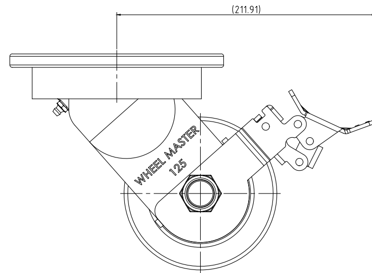
WXT-125SFBK-TYPE B
