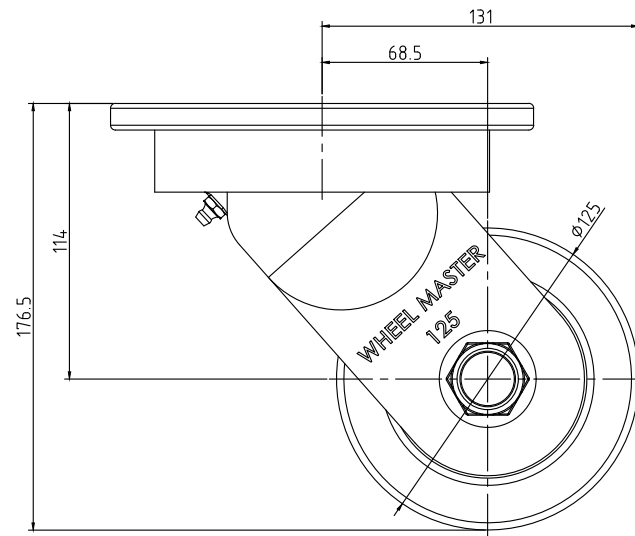
WXT-125SF
