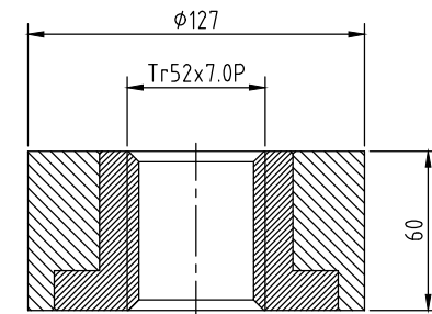
W-TYPE (용접형)
