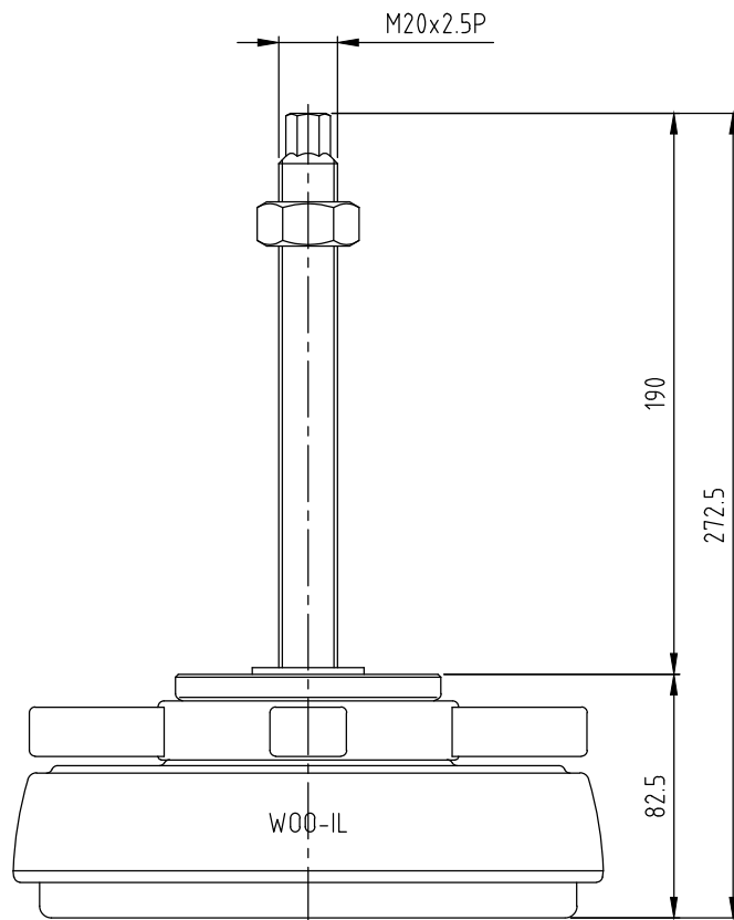
WSH200-M20x190L
