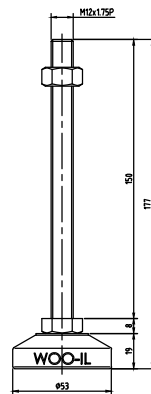
MFZ53-M12-150
