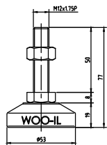
MFZ53-M12-50
