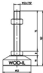
MFZ53-M12-75
