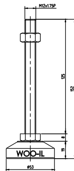
MFZ53-M12-125
