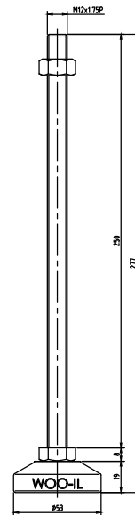
MFZ53-M12-250
