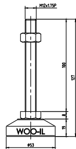
MFZ53-M12-100
