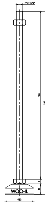
MFZ53-M12-300
