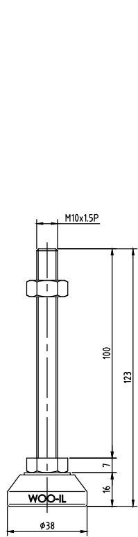
MFT38-M10100
