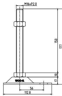
ABL76-M16-150
