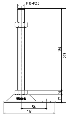
ABL76-M16-180
