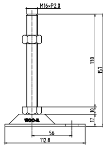
ABL76-M16-130
