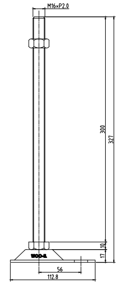
ABL76-M16-300
