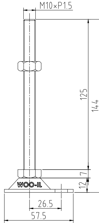
ABL42-M10-125
