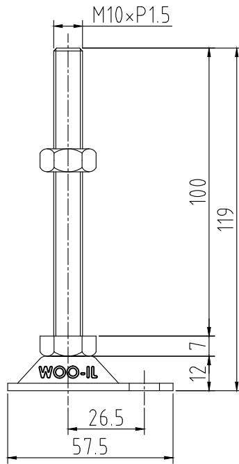
ABL42-M10-100
