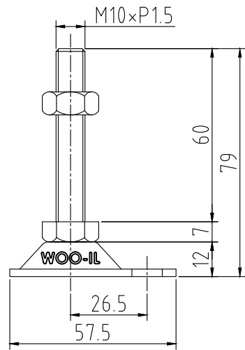
ABL42-M10-60
